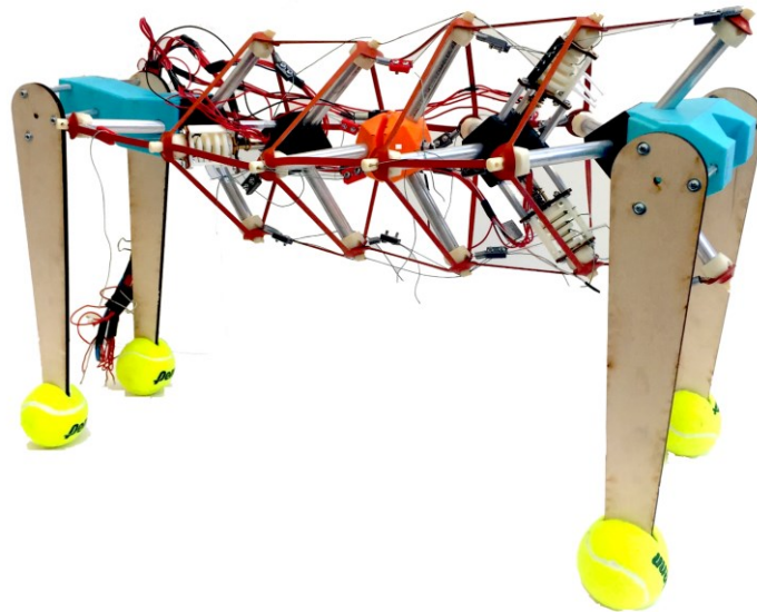
Fig.: The quadruped robot with a tensegrity spine
