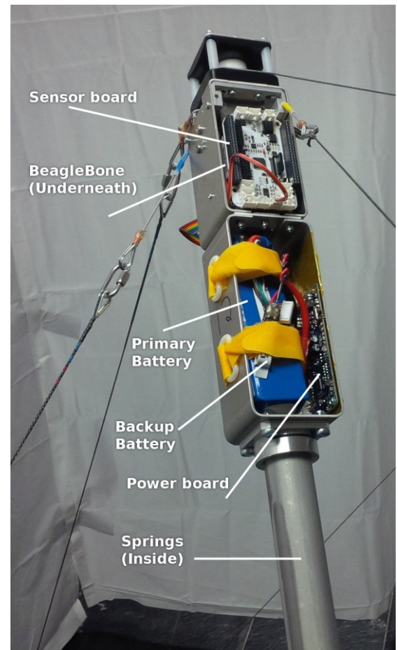
Fig.: Spherical Tensegrity Robotics Mechanisms in locomotion
