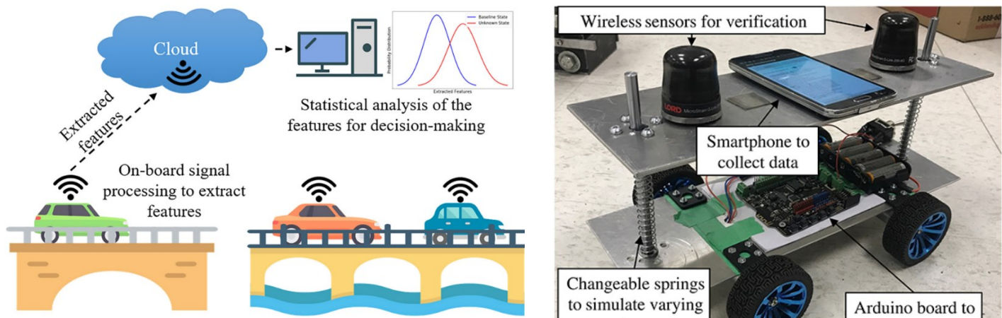
Fig.: Overview of the damage detection technique.
