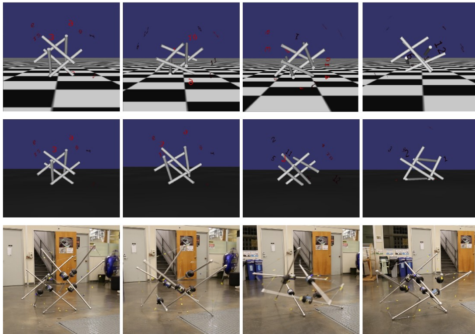
Fig.: Spherical Tensegrity Robotics Mechanisms in locomotion
